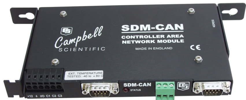
FIGURE 1-1. SDM-CAN CAN-Bus Interface
